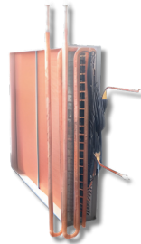
Marine Air Conditioner Heat Exchanger
